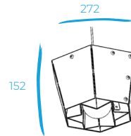
PWCF-301 Barnacle lamp ceiling single, small, 1,35 kg
