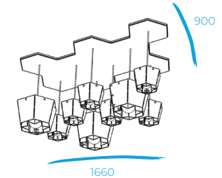
PWCF-304 Barnacle lamp ceiling panel 3 lamps tall, 6 lamps small
